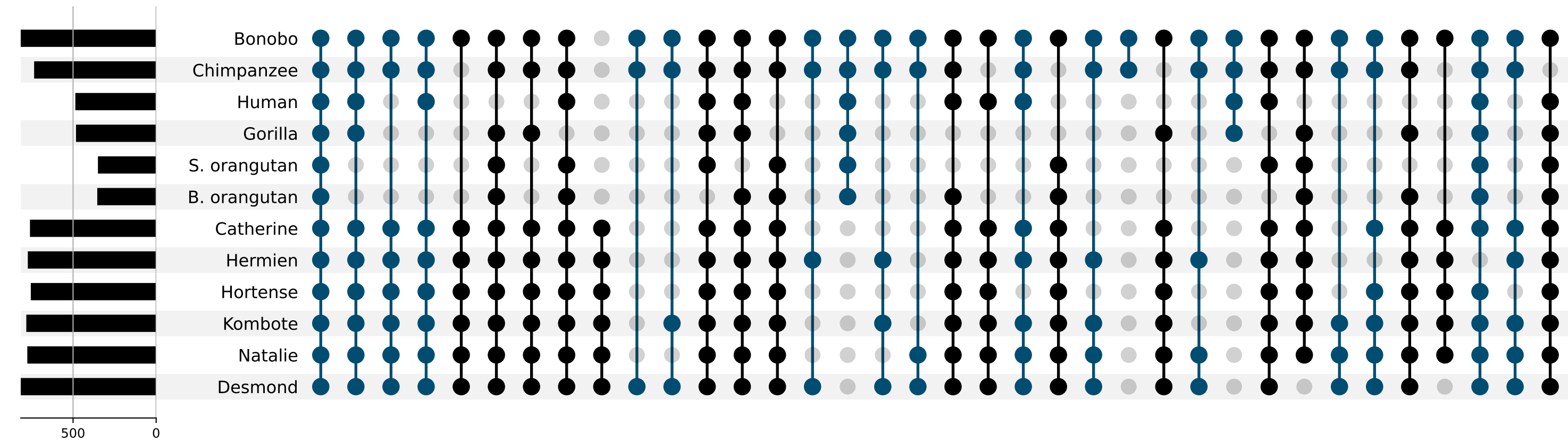
Total # of NUMTs in species
