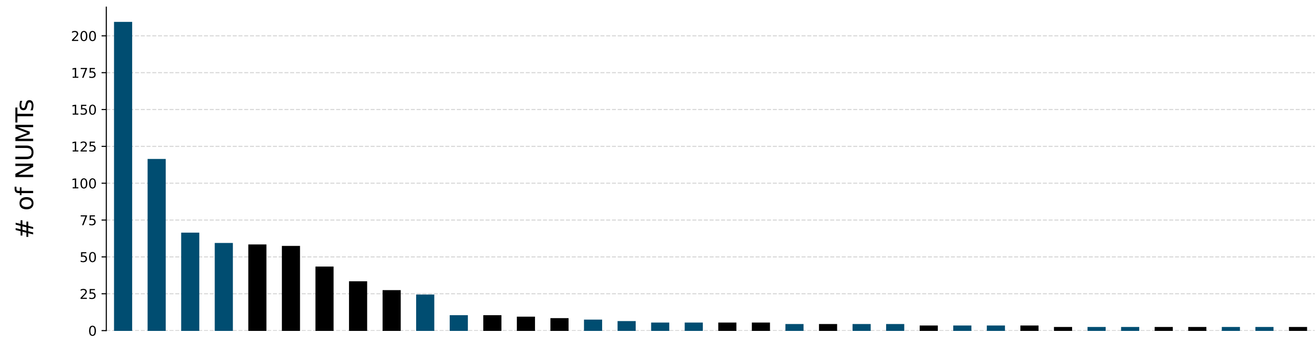
Number of NUMTs shared among species
